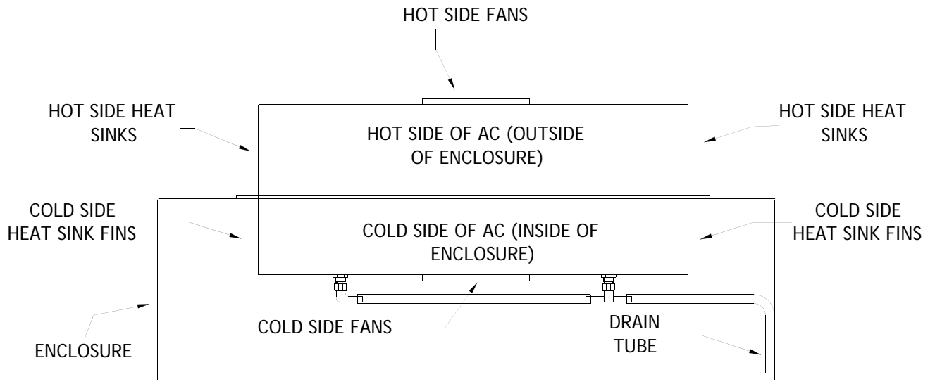
HORIZONTAL INSTALLATION OF 1000 BTU UNIT WITH INTERNALLY MOUNTED DP-146H DRIP PAN AND DRAIN TUBE
