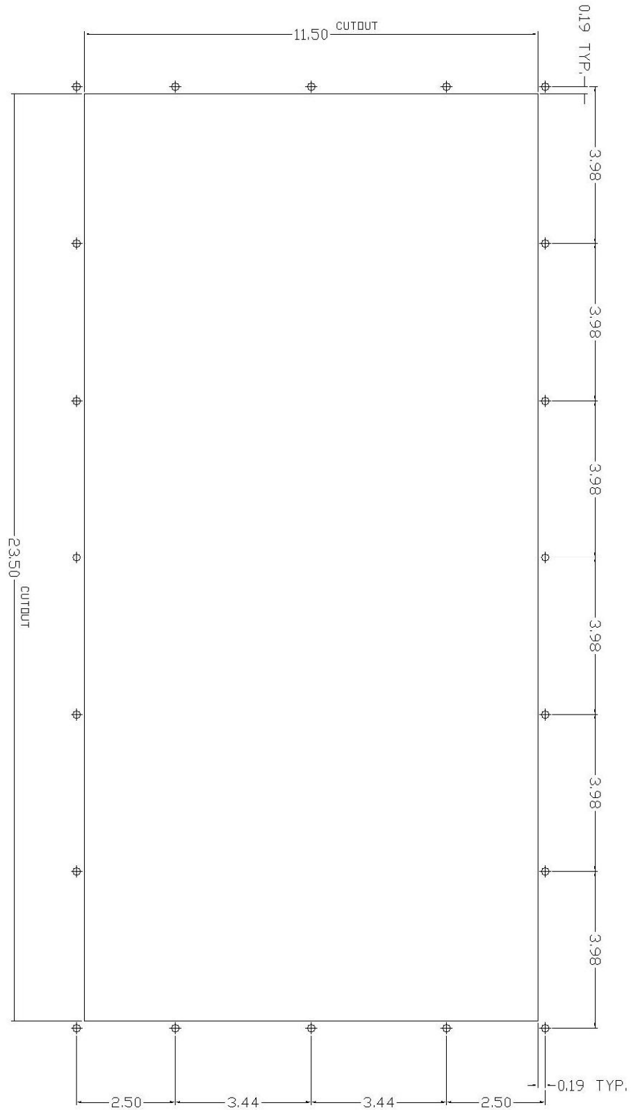
Enclosure cutout for 1000 BTU air conditioner EXTENSION FRAME ONLY
