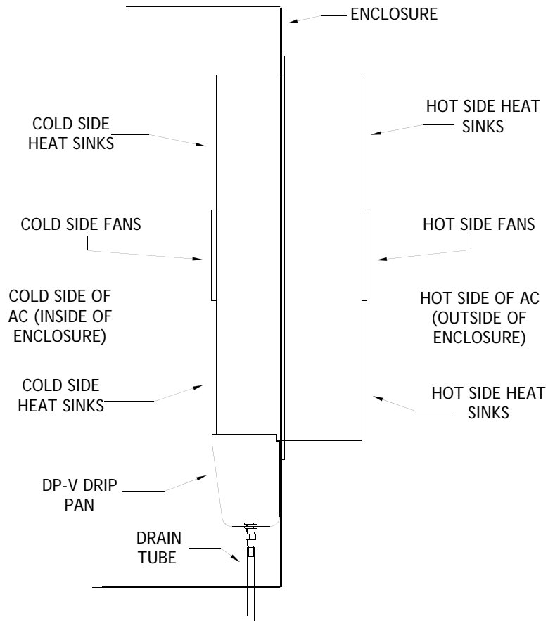
VERTICAL INSTALLATION OF 1000 BTU UNIT WITH DP-V VERTICAL DRIP PAN AND DRAIN TUBE
